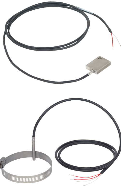
Fig. top: Model TR50 with metal contact block
