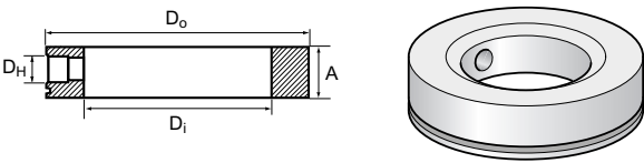
Figure 36: Flushing Connection Rings
