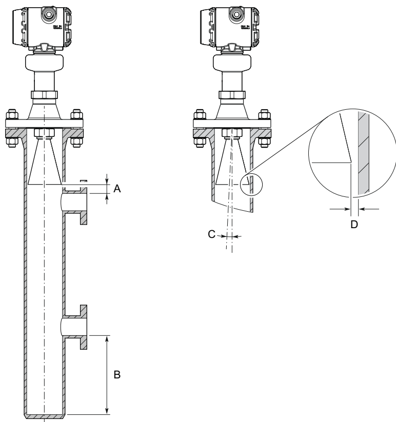
Figure 24: Chamber Requirements
