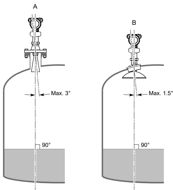
Figure 18: Inclination
