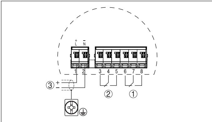
Fig. 16: Wiring plan, receiving unit - VEGAMIP (receiver)
