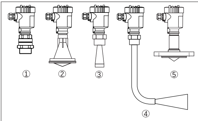
Fig. 6: Antenna versions
