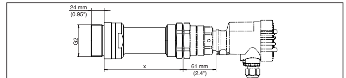
Fig. 23: Mounting adapter with ceramic cover for VEGAMIP - threaded version with PTFE cover
