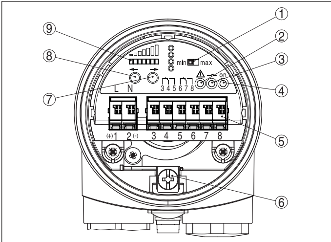
Fig. 17: Electronics module MPE60R receiver unit - Relay output
