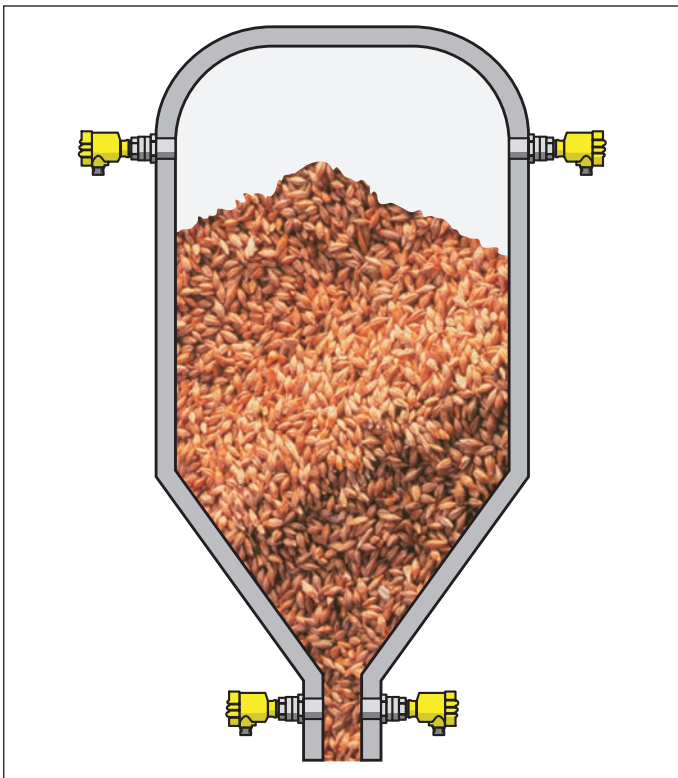
Fig. 12: Level detection in a bulk solids vessel
