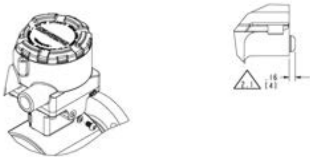
Figure 21: M1 Housing Option Detail
