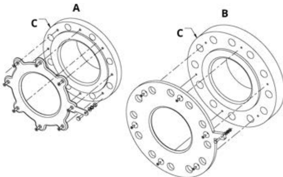
Figure 24: 8705-M Flanged Sensor ½ in. to 36 in. (DN 15 mm to 900 mm) Lining Protectors—(P ≤ Class 900)
