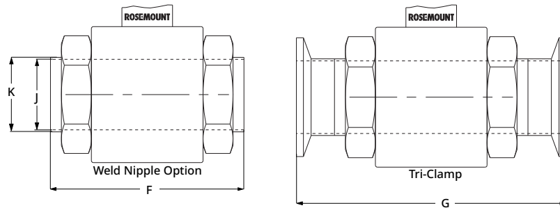
Figure 29: 8721 Hygienic (Sanitary) Sensor Weld Nipple and Tri-Clamp
