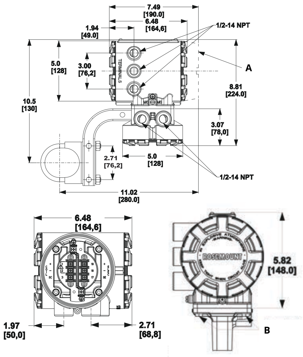
Figure 14: 8732 Field Mount Transmitter Dimensions
