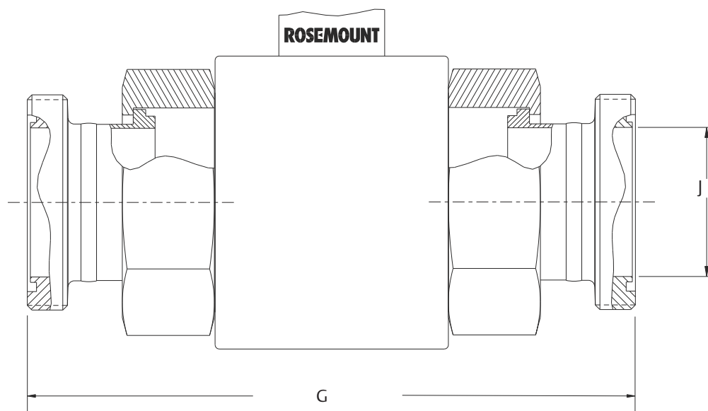
Figure 34: 8721 Hygienic (Sanitary) Sensor SMS1145
