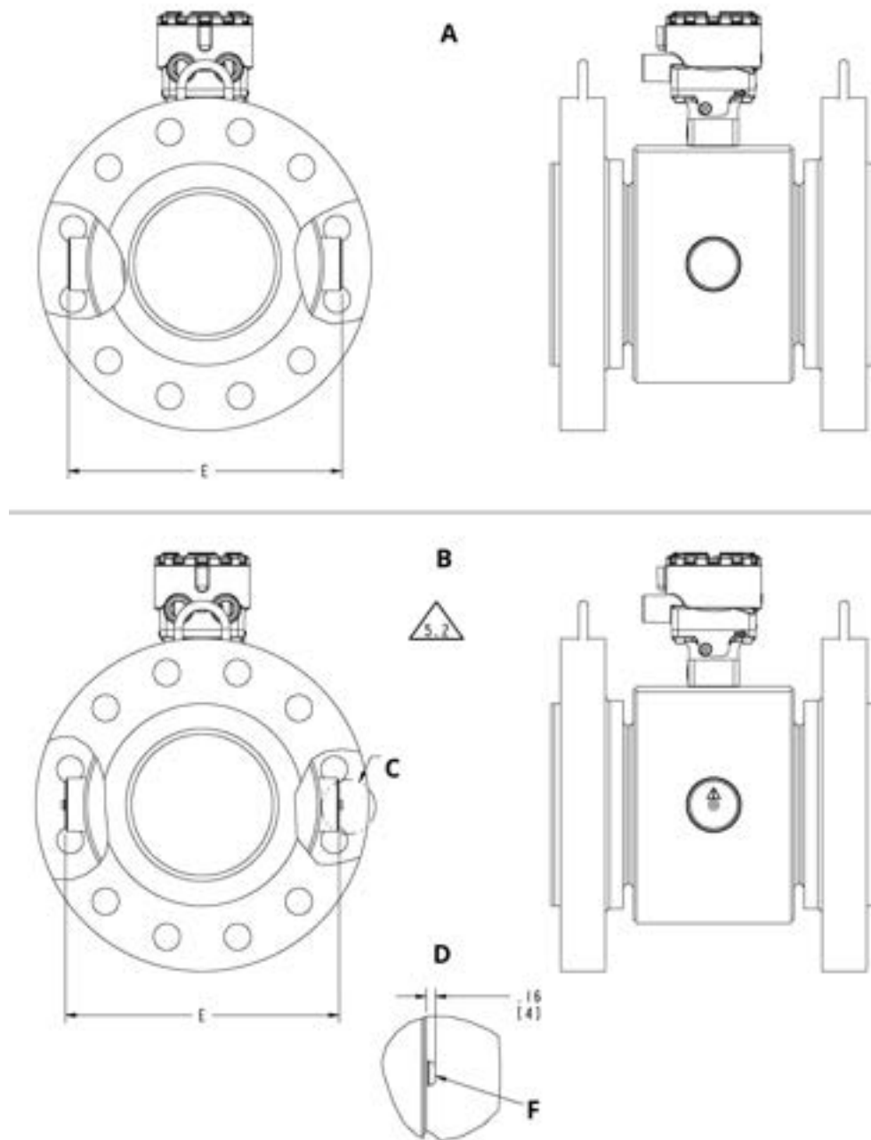
Figure 23: 8705-M Flanged Sensor ½ in. to 36 in. (DN 15 mm to 900 mm) M2/M4 Coil Housing (P ≤ Class 2500)
