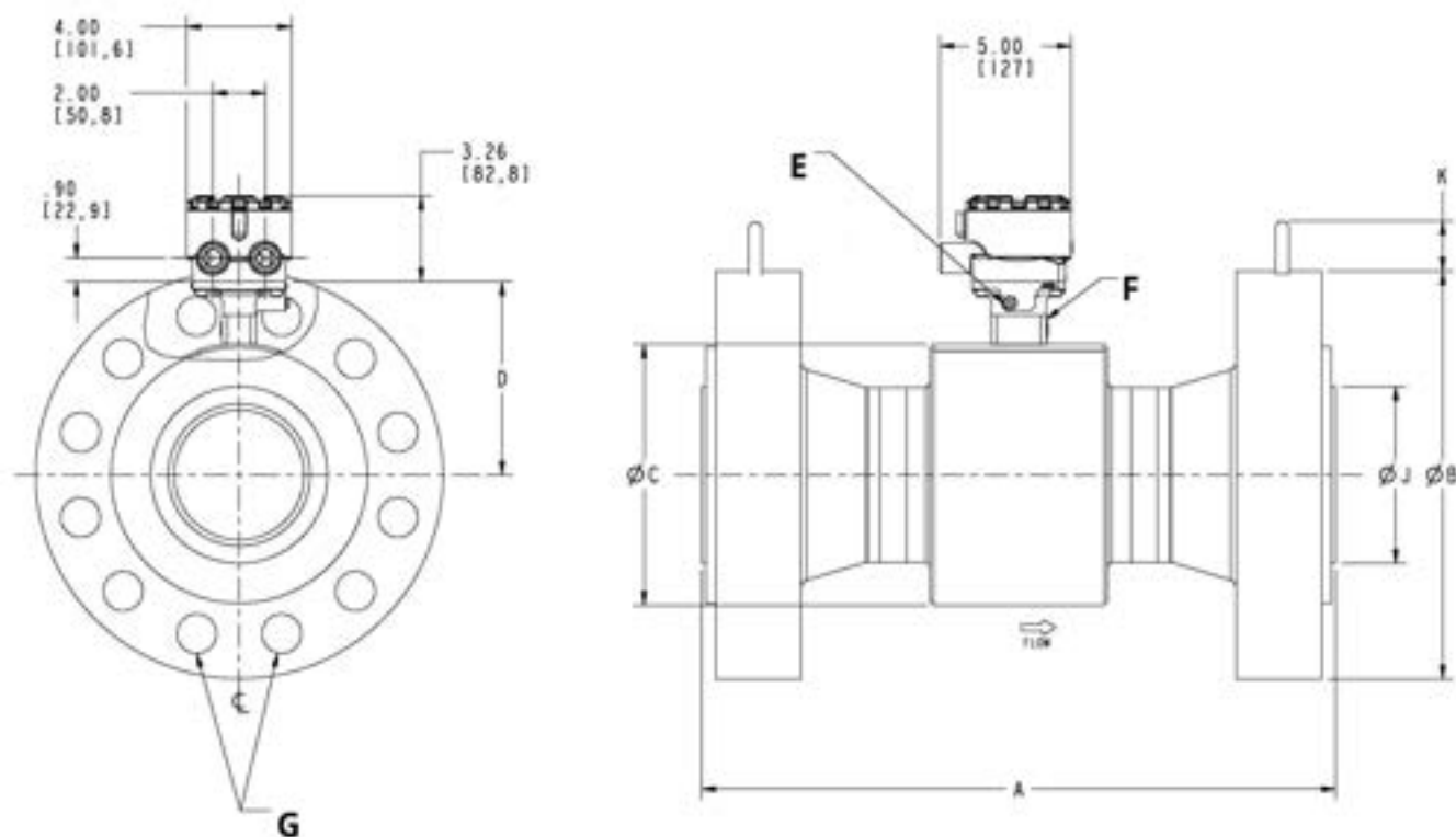
Figure 22: 8705-M Flanged Sensor 1 in. to 24 in. (DN 25 mm to 600 mm) Weld-neck Flange—(P ≤ Class 2500)
