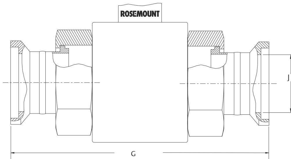
Figure 35: 8721 Hygienic (Sanitary) Sensor Cherry Burrell I-Line
