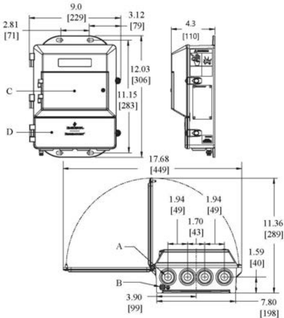
Figure 13: 8712 Wall Mount Transmitter Dimensions
