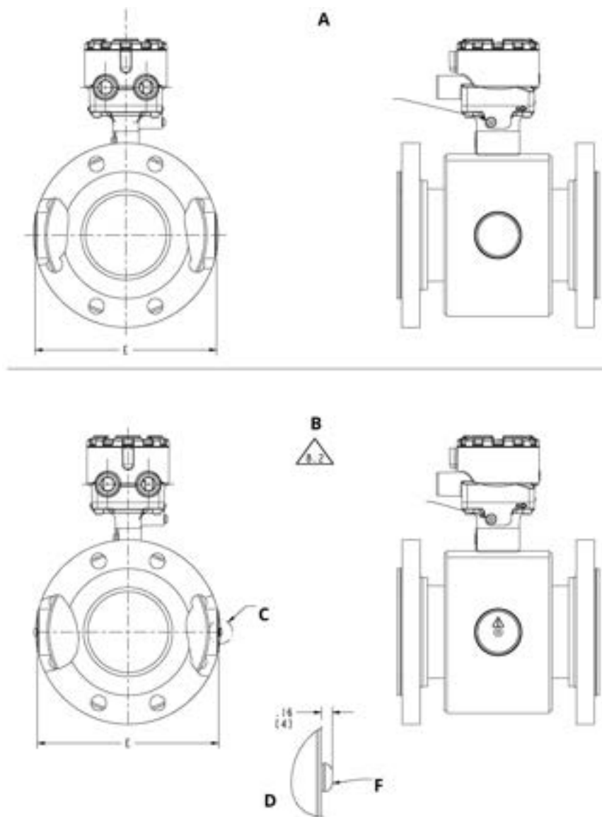
Figure 19: 8705-M Flanged Sensor ½ in. to 36 in. (DN 15 mm to 900 mm) M2/M4 Coil Housing (P ≤ Class 600 derated)
