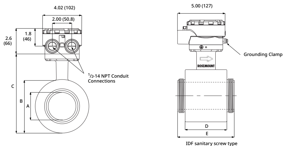
Figure 28: 8721 Hygienic (Sanitary) Sensor ½ in. to 4 in. (15 mm to 100 mm)
