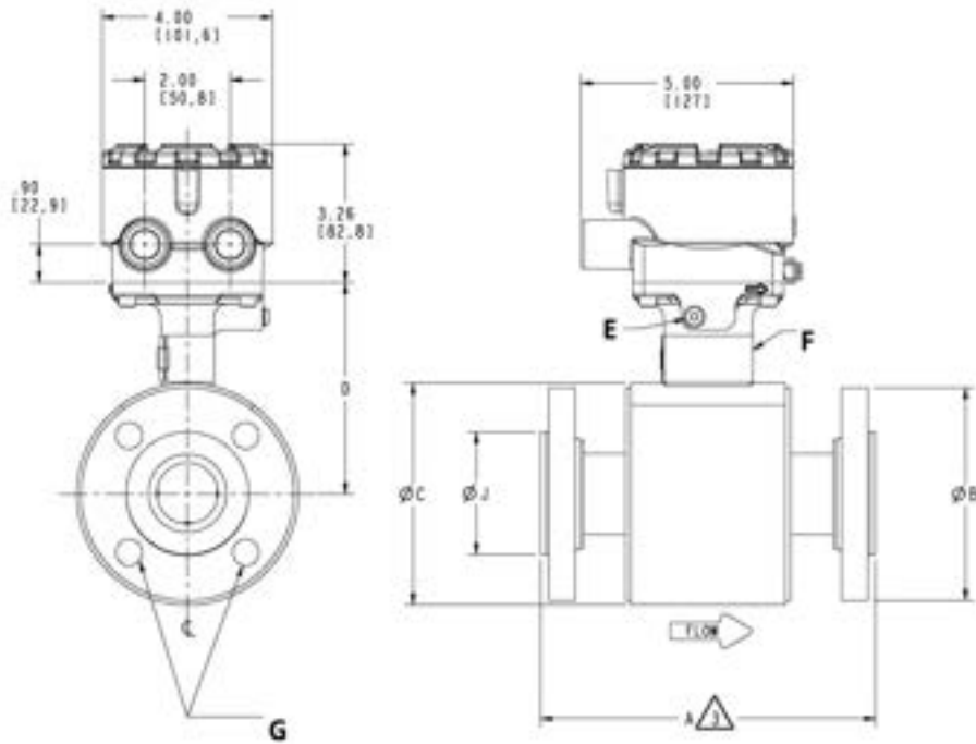
Figure 20: 8705-M Flanged Sensor ½ in. to 24 in. (DN 15 mm to 600 mm) Slip-on Flange—High Pressure ( P \leq \text{Class } 900 )
