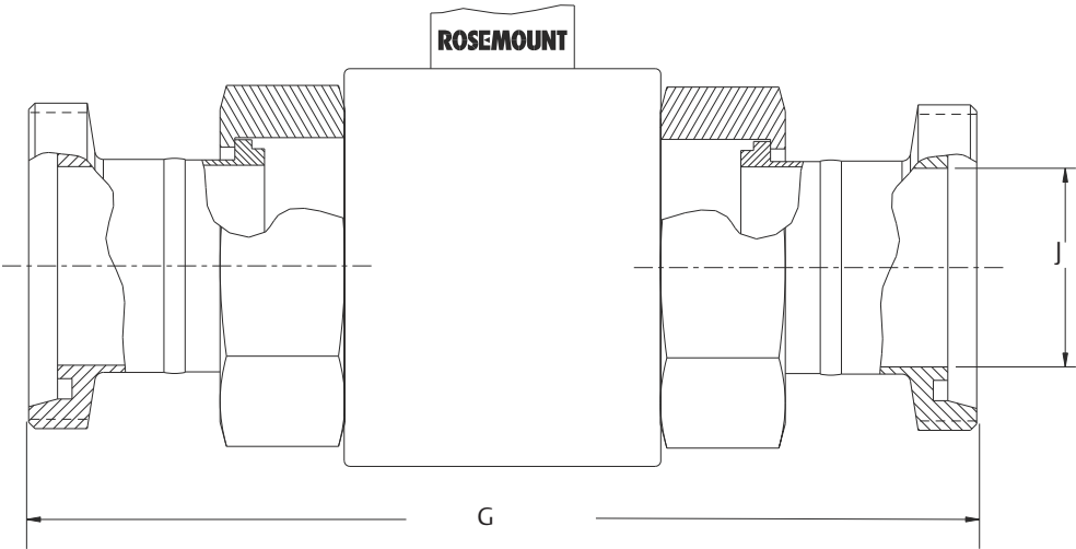
Figure 31: 8721 Hygienic (Sanitary) Sensor DIN 11851 (Metric)
