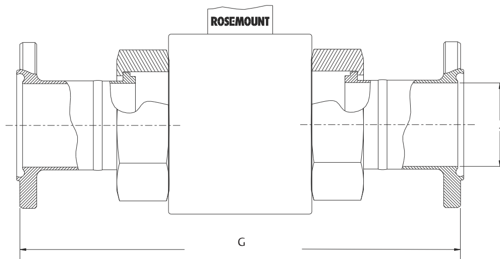
Figure 33: 8721 Hygienic (Sanitary) Sensor DIN 11864-2
