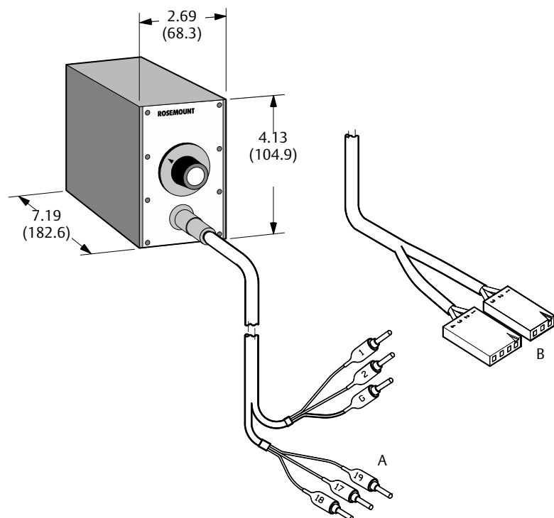
Figure 36: 8714D Magnetic Flow Meter Simulator—Calibration Standard
