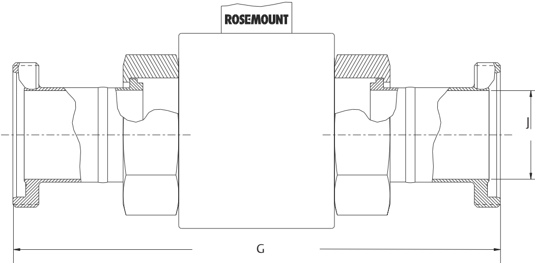
Figure 32: 8721 Hygienic (Sanitary) Sensor DIN 11864-1
