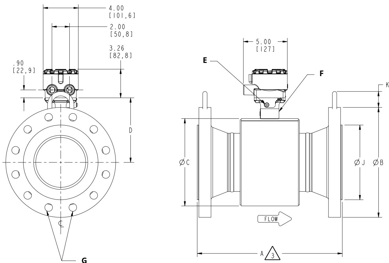
Figure 18: 8705-M Flanged Sensor ½ in. to 36 in. (DN 15 mm to 900 mm) Weld-neck Flanges—(P ≤ Class 600 derated)
