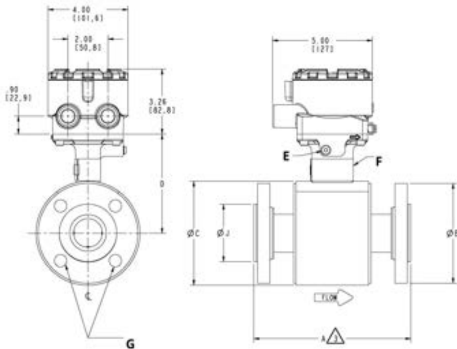
Figure 15: 8705-M Flanged Sensor 0.5 in. to 2.5 in. (DN 15 mm to 65 mm) Slip-on Flanges—Low Pressure (P < Class 300)
