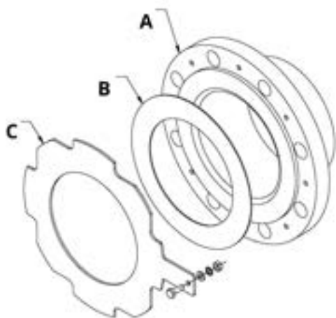
Figure 25: 8705-M Flanged Sensor ½ in. to 36 in. (DN 15 mm to 900 mm) Ground Rings—(P ≤ Class 900)
