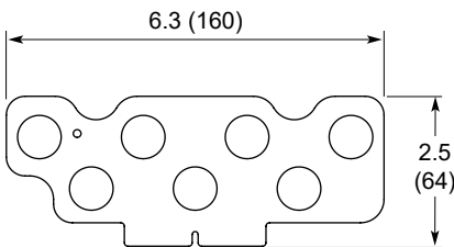
Figure 7: Support Plate
