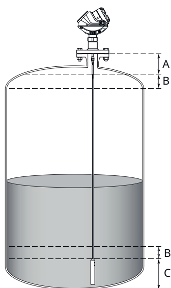
Figure 4: Blind Zones
