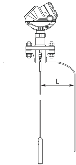
Figure 26: Free Space Requirement
