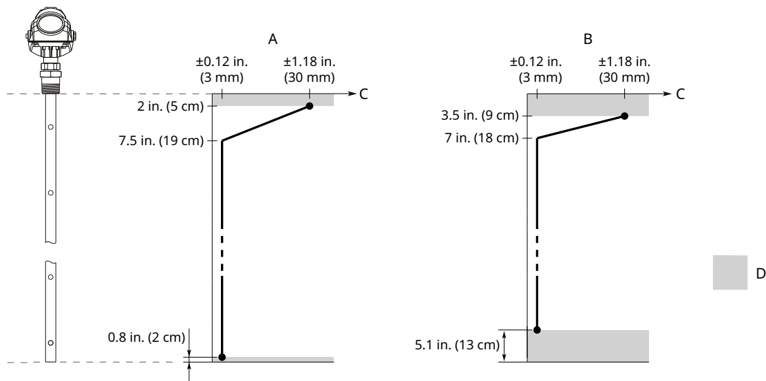
Figure 6: Accuracy Over Measuring Range for Coaxial Probe
