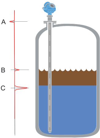
Figure 1: Measurement Principle
