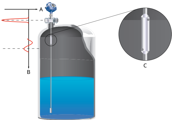
Figure 12: Verification Reflector
