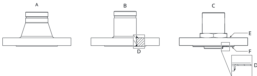
Figure 52: Flange Connection
