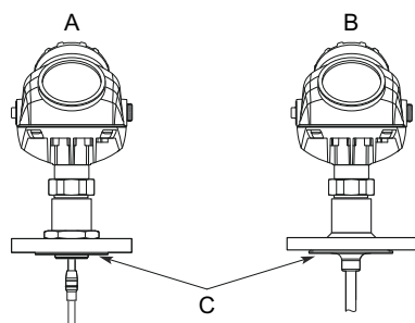
Figure 20: Protective Plate
