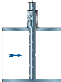
1 - 2 = Attacco al processo filettato 1" NPT-M ANSI B1.20.1 completo di manicotto a saldare. Process connection threaded 1" NPT-M ANSI B1.20.1 complete of welding coupling.
